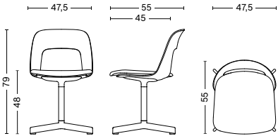
LAYOUT CHAIR 133 Width 47,5 cm Depth 55 cm Height 79 cm Seat height 48 cm Weight 8,8 kg
