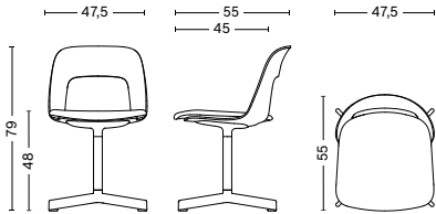
LAYOUT CHAIR 134 Width 47,5 cm Depth 56 cm Height 80 cm Seat height 48 cm Weight 9,2 kg
