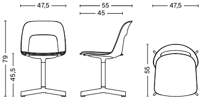
LAYOUT CHAIR 132 Width 47,5 cm Depth 55 cm Height 79 cm Seat height 45,5 cm Weight 8,3 kg
