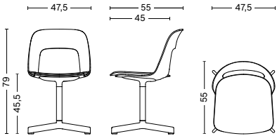
LAYOUT CHAIR 131 Width 47,5 cm Depth 55 cm Height 79 cm Seat height 45,5 cm Weight 8,4 kg
